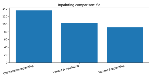
5(a) FID comparison
