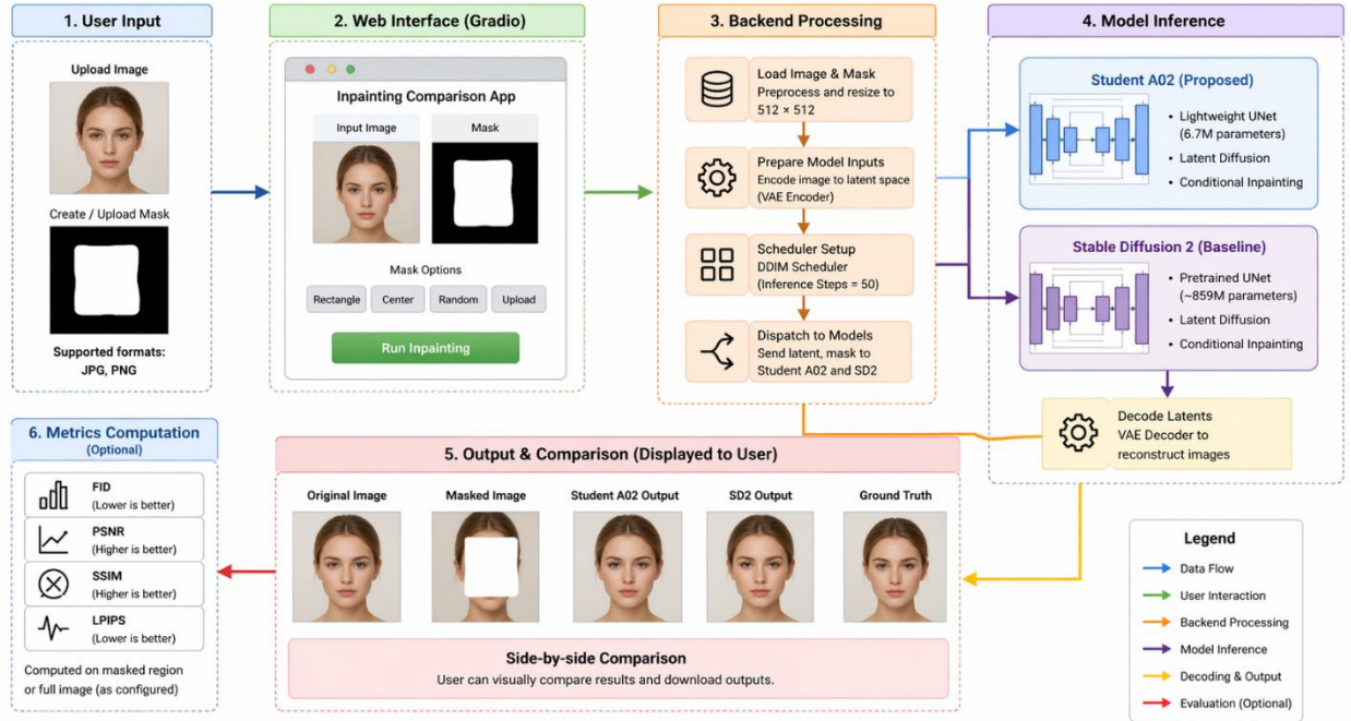
Figure 2 End-to-end deployment workflow for Student A02 and Stable Diffusion 2 comparison.
