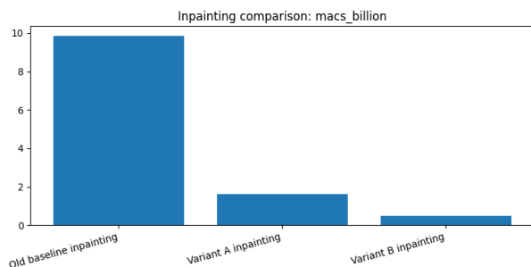
5(c) Computational cost (MACs, billions)
