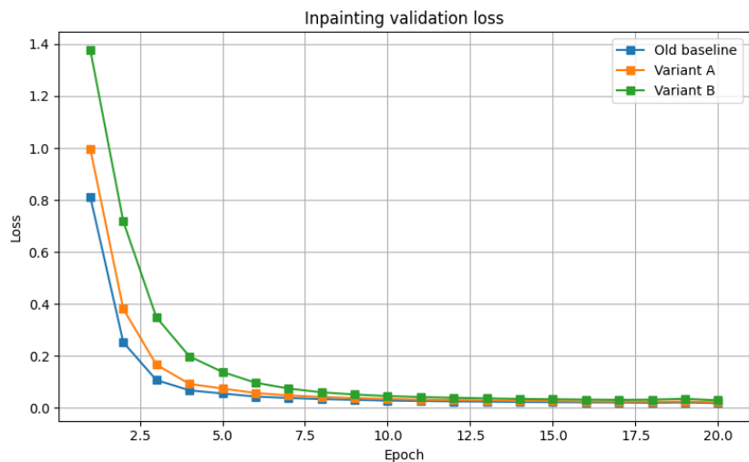
Figure 4 Validation loss curve for CelebA inpainting variants.
