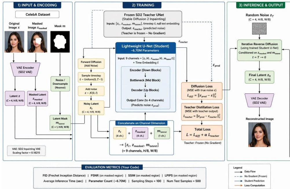
Figure 1 Proposed lightweight latent diffusion inpainting architecture for Student A02.
