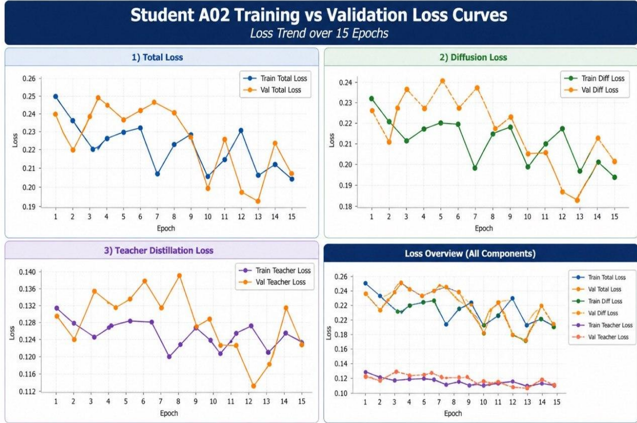
Figure 6. Training and validation loss curves of the Student A02 model across different loss components.
