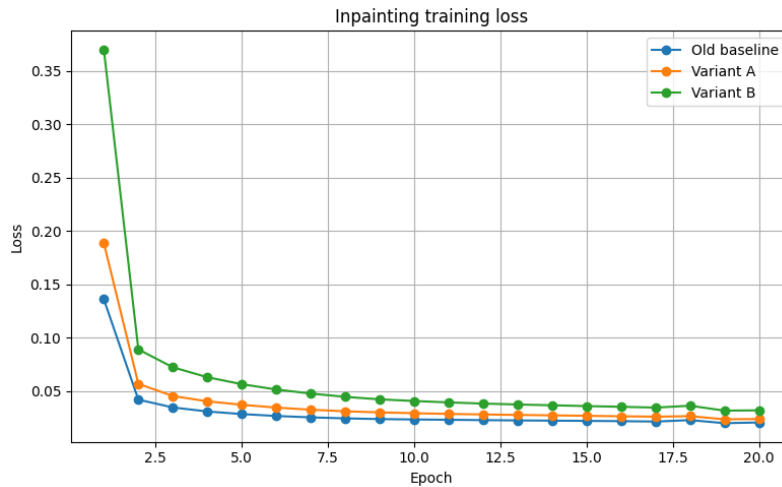
Figure 3 Training loss curve for CelebA inpainting variants.
